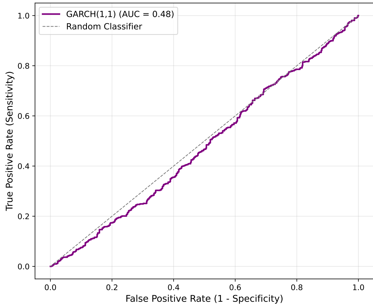
ROC Curve — GARCH(1,1) Directional Forecast
